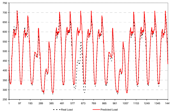
Figure 5: Real and Predicted Loads – 01/09/2005 to 15/09/2005
