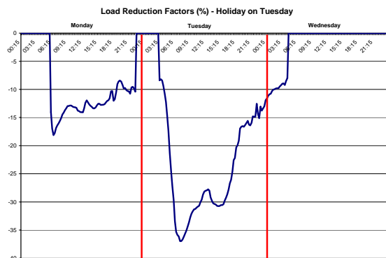
Figure 1: Load Reduction Factors – Holiday Occurring on Tuesday
