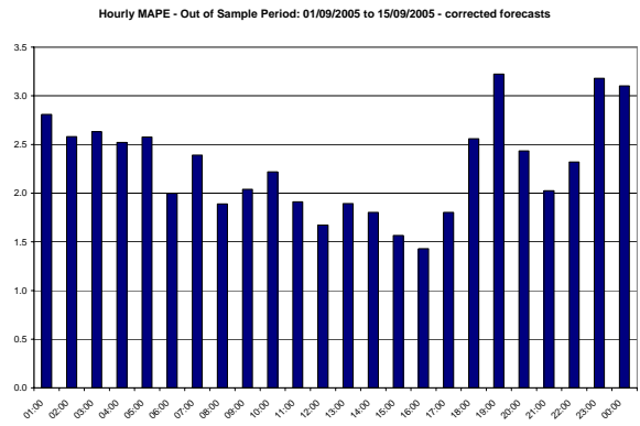
Figure 7: Hourly Average MAPEs – Corrected Forecasts
