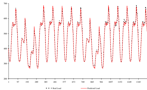
Figure 2: Real and Predicted Loads – 15/07/2005 to 29/07/2005
